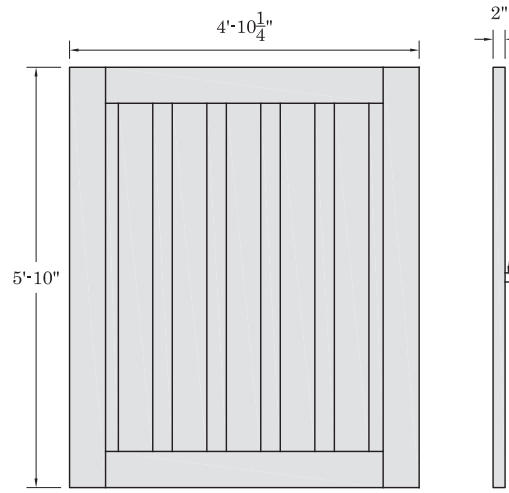
STANDARD 10' X 6' DOUBLE GATE PANEL
