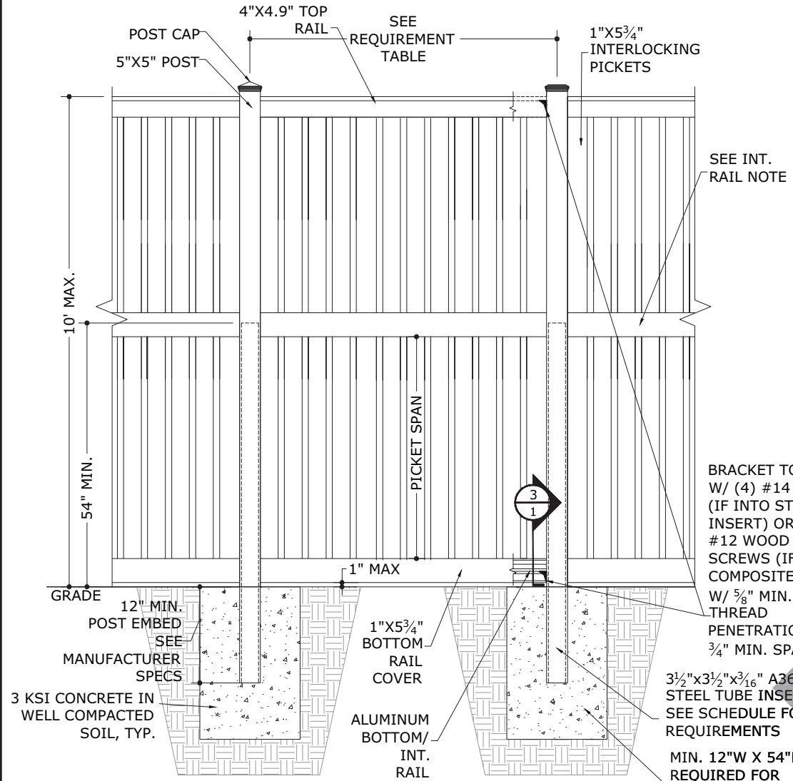
10' COMPOSITE FENCE SCALE: NTS ELEVATION VIEW
