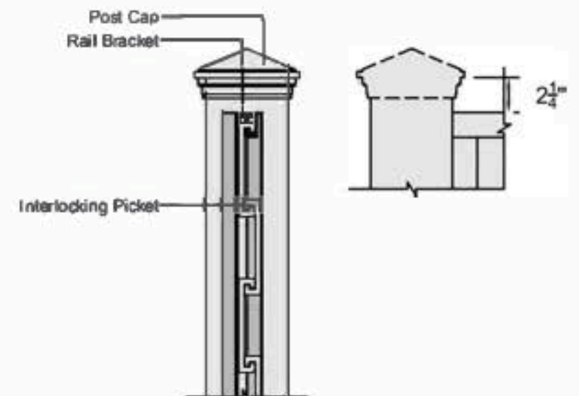
Post Profile: Cut View / Elevation View
