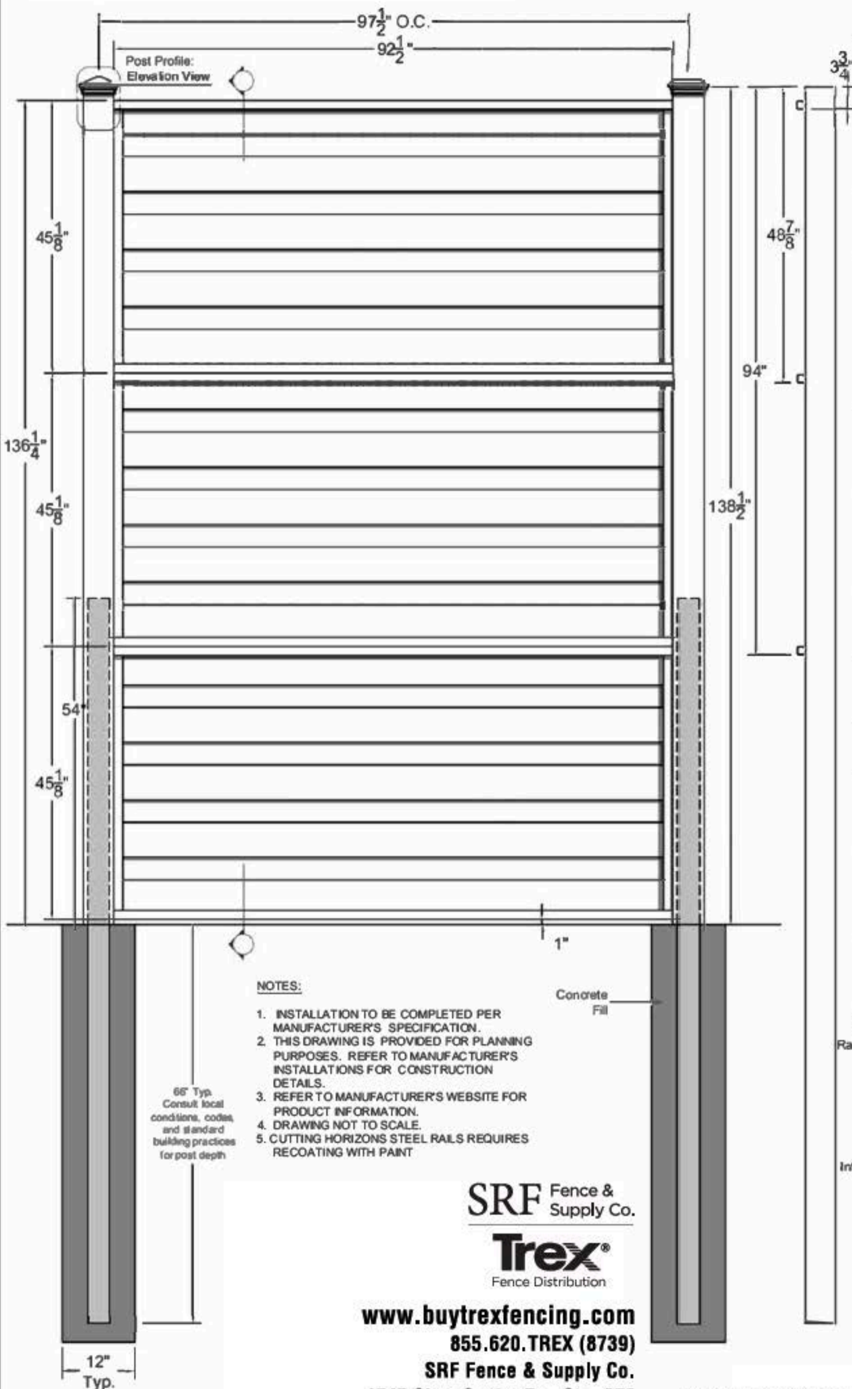
Post Profile: Cut View / Elevation View
