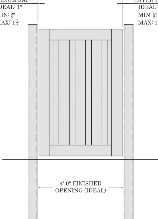
STANDARD 4' X 6' WALK GATE PANEL
