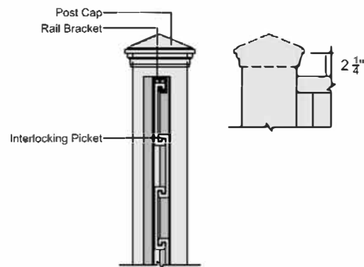
Post Profile: Cut View / Elevation View
