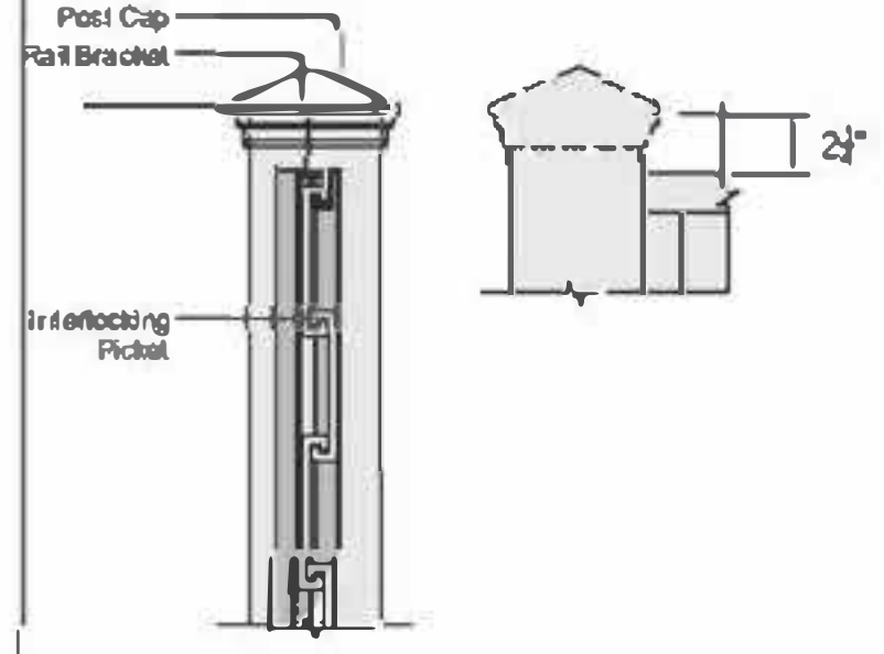
Post Profile: Cut View / Elevation View
