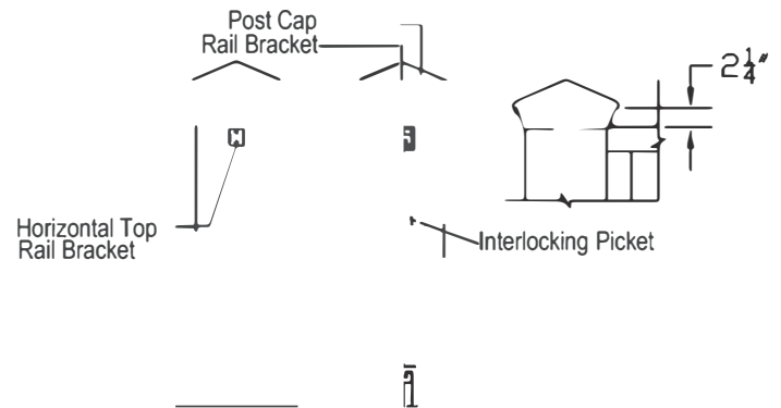
Post Profile: Cut View / Elevation View
