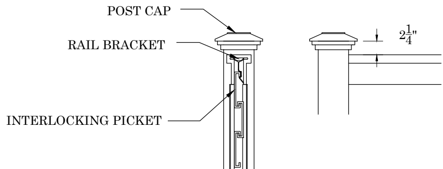
POST PROFILE: CUT VIEW/ELEVATION VIEW
